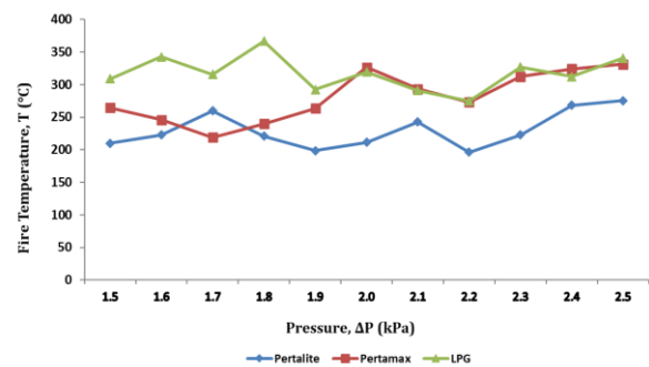
Figure 2. Relation of pressure ( \Delta P ) to fire temperature ( ^{\circ}C ) at gasoline fuel (Peralite, Pertamina) and LPG fuel
